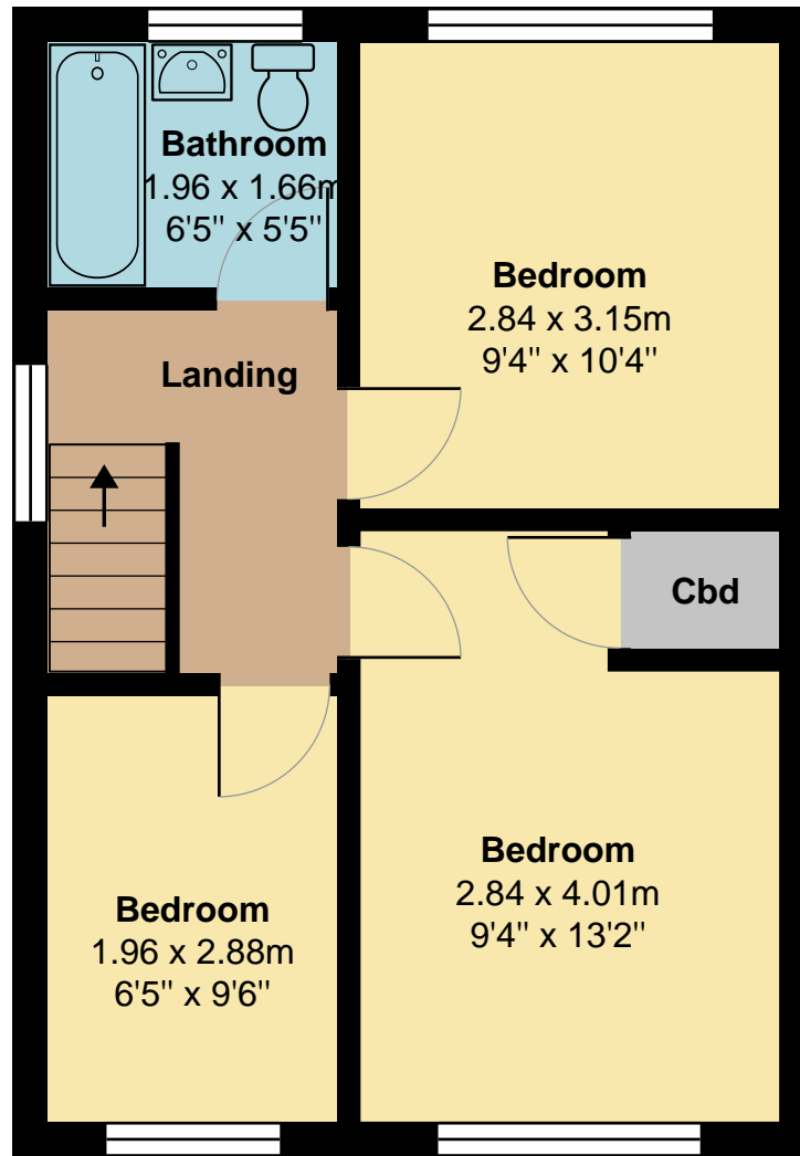
First Floor
